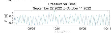
Figure 2a (top) shows the raw pressure data received from the sensor plotted against time. Figure 2b (bottom) shows the data after high pass filtering to remove low frequency (tides and atmospheric effects.).
