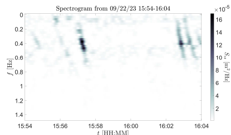
Figure 5 is a spectrogram that contains 5 wake signatures. 3 on the left and a double signature on the right.
