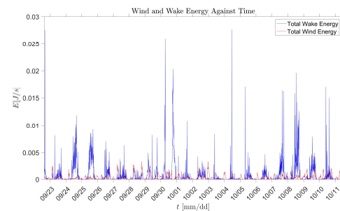
Figure 8 displays the total energies for wind (red) and wakes (blue) for every 10-minute spectrogram analyzed by imgNet.
